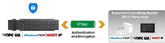
Figure 6. PLC Communication Secured with IPSec
