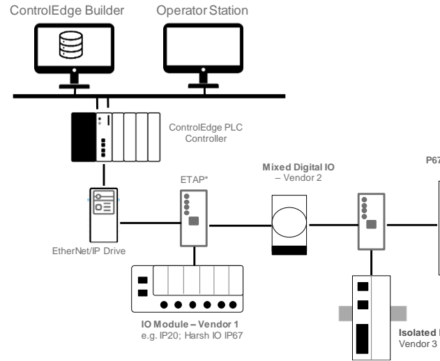
Figure 7 – Multivendor EtherNet/IP device and I/O module connectivity
