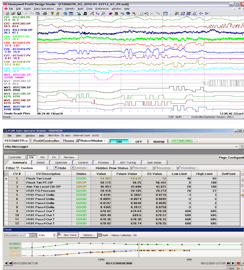
Figure 2. Profit Stepper R320 is a powerful tool designed for automated data collection and step testing.
